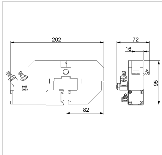
Pneumatic grips type 8097, Fmax 200 N, overview
