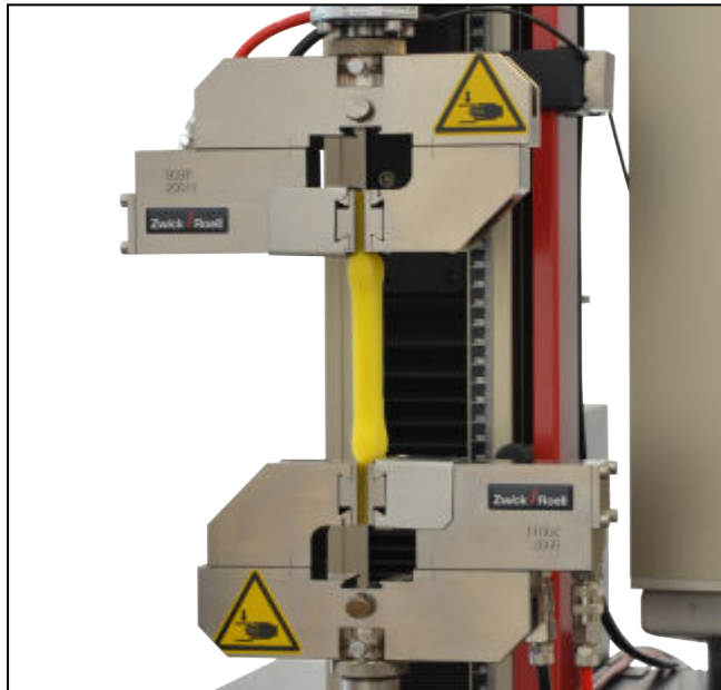
Pneumatic grips type 8097, Fmax 200 N, opposing jaw with stepped adjustment
